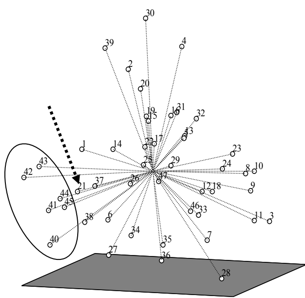
Figure 5. Three-dimensional plot of principal coordinate analysis using 47 accessions of Lansium domesticum 'duku' and L. domesticum 'kokosan'. The numbers plotted represent individual sample and corresponds to notes in Figure 2. Dotted arrow: Lansium sp. from Ceram. Circle correspond to the grouping at Figure 4 as Duku Bengkulu. Vertical line axis Z.
